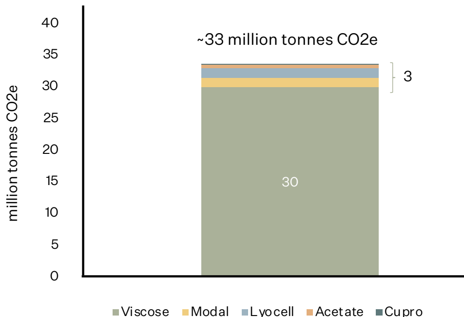
Figure 6: GHG impact for MMCFs for the 2019 baseline. This impact considers the following sectors only: fashion and apparel, home textiles and footwear'. Sources: Production data - Textile Exchange's Preferred Fiber and Material Market Report, 2022; Sector split data - Textile Exchange Data and Technology Team research, 2021; Results were calculated using Higg MSI 3.3 data at Higg.org. Retrieved by Textile Exchange in March 2022
