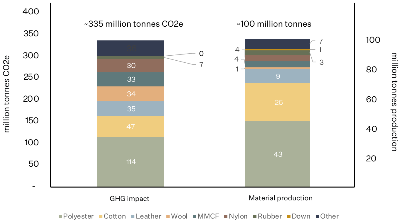
Figure 1: GHG impact across and production volumes for fiber and material categories for the 2019 baseline. 1 This chart considers the following sectors only: fashion and apparel, home textiles and footwear and does not consider total global production (as published in the Preferred Fiber and Material Market Report. Sources: Production data – Textile Exchange’s Preferred Fiber and Material Market Report, 2022; Sector split data – Textile Exchange Data and Technology Team research, 2021; Results were calculated using Higg MSI 3.3 data at Higg.org. Retrieved by Textile Exchange in March 2022
